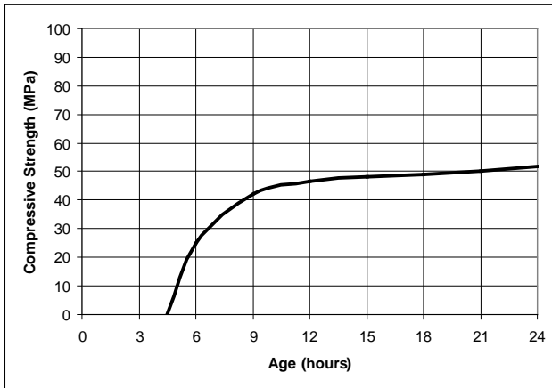
Typical Development of Compressive Strength - LUMNITE MG ®
